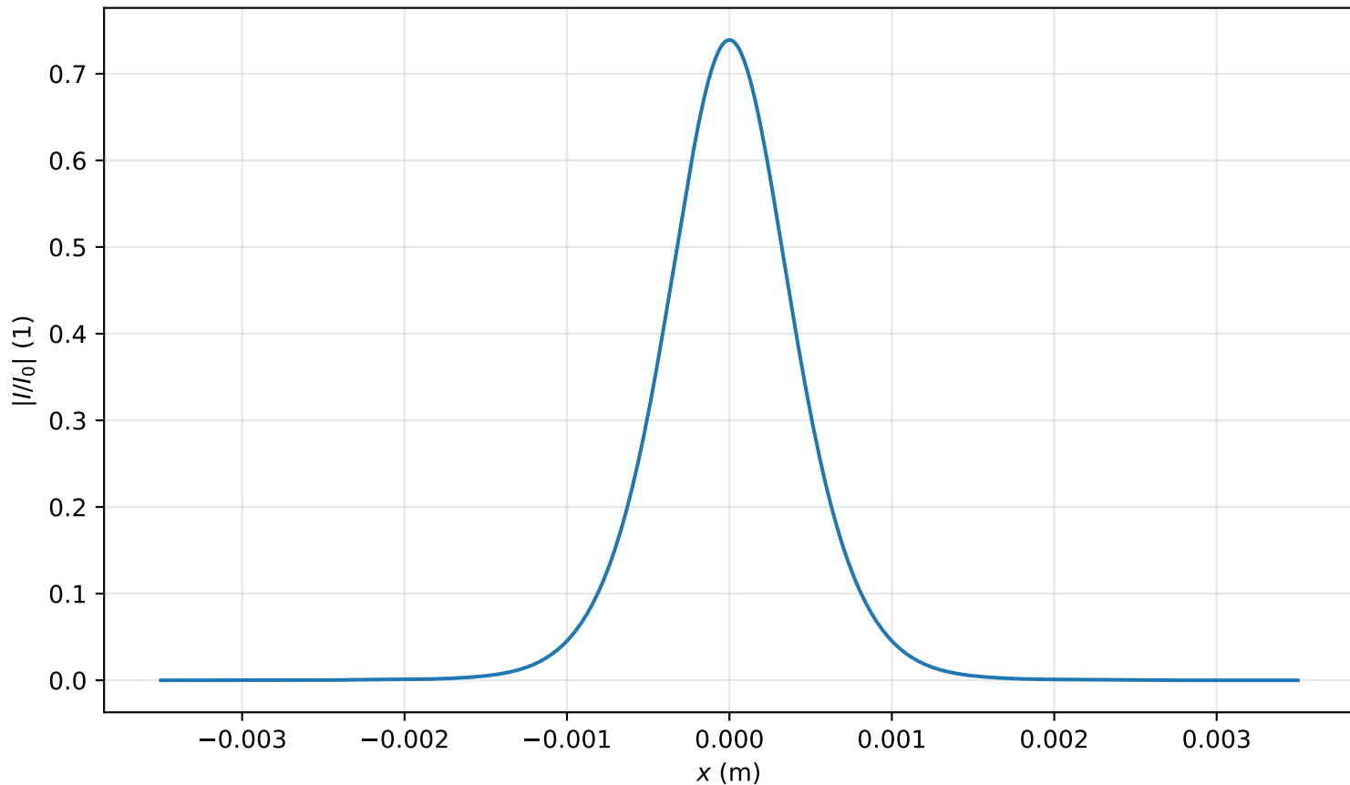
Intensity profile I(x, y = 0, z = 3.423m)/I_0 , P_{in}=0.7P_{cr} , artificial time
